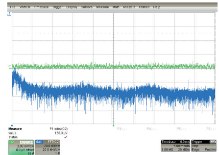
PS1215 -15V typical output noise - AC coupling - BW160kHz
