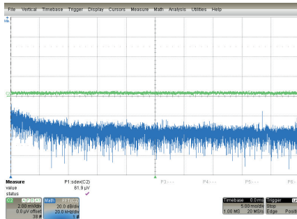
PS1215 +15V typical output noise - AC coupling - BW160kHz
