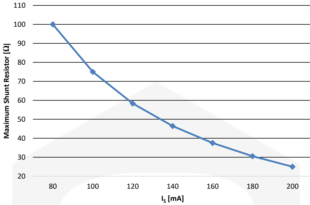
Figure 15: CT-400 maximum external shunt resistor ( Current version only)
