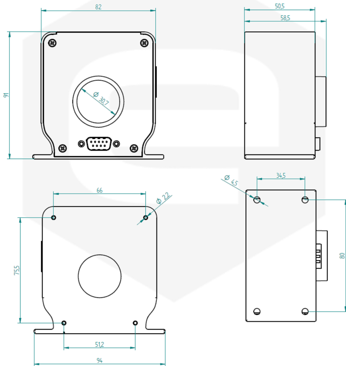
Figure 16: Mechanical drawings
