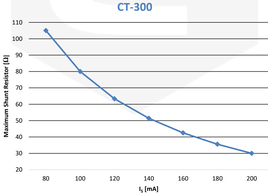
Figure 14: CT-300 maximum external shunt resistor ( Current version only)
