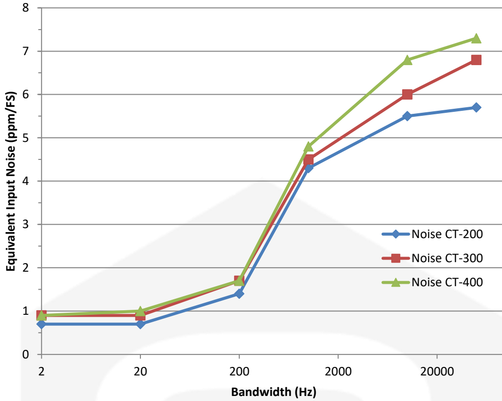
Figure 12: Equivalent input noise graph (typical values)
