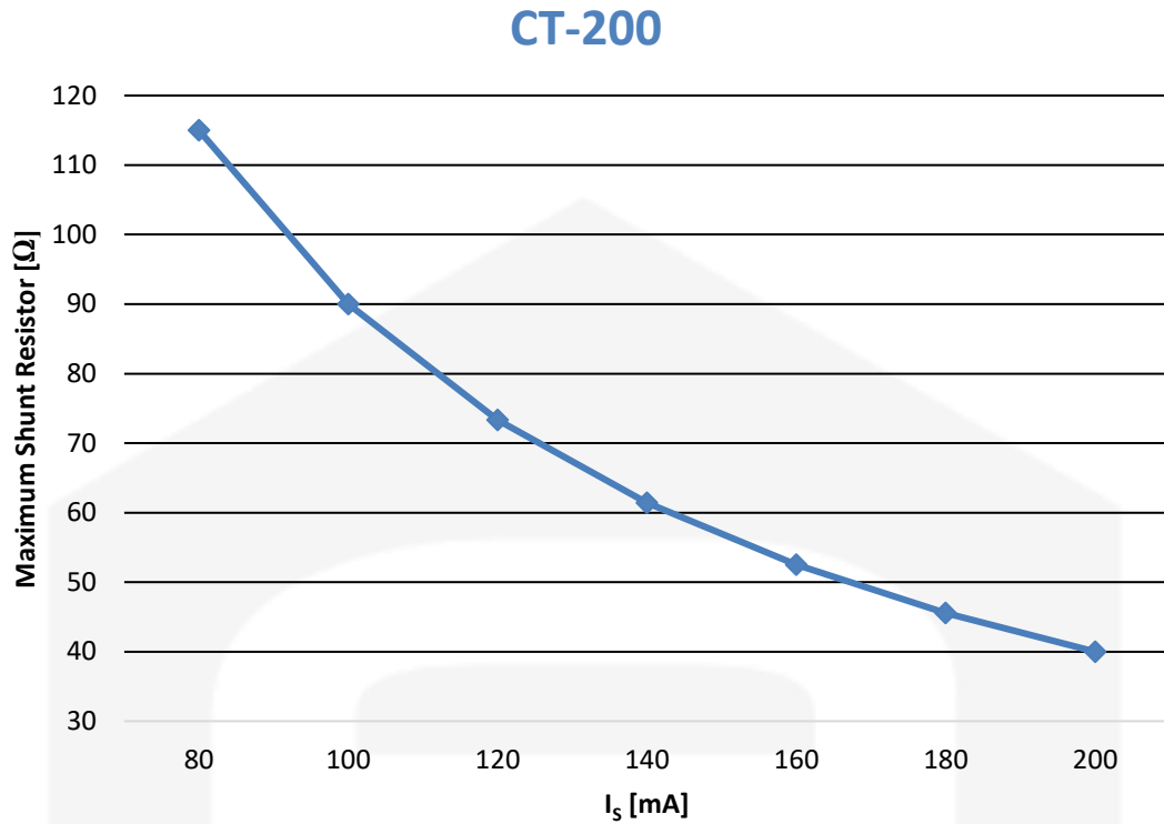
Figure 13: CT-200 maximum external shunt resistor ( Current version only)
