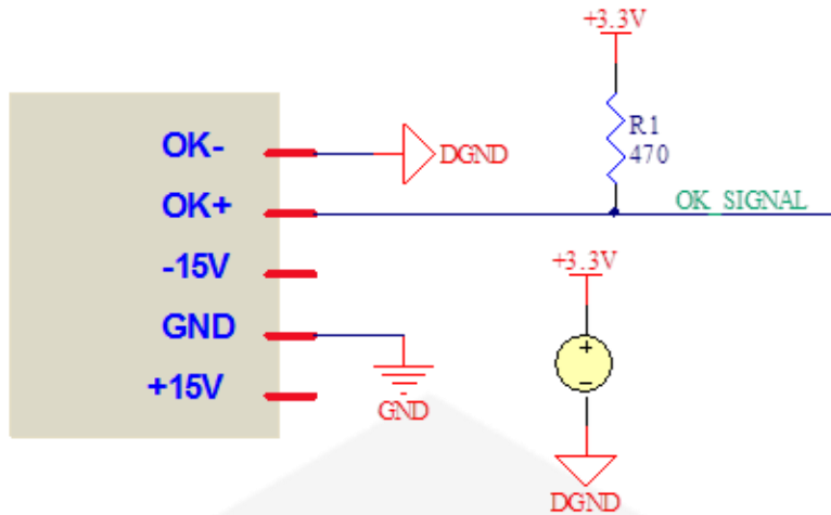
Figure 6: OUT OK signals connections as digital interfacing to +3.3V
