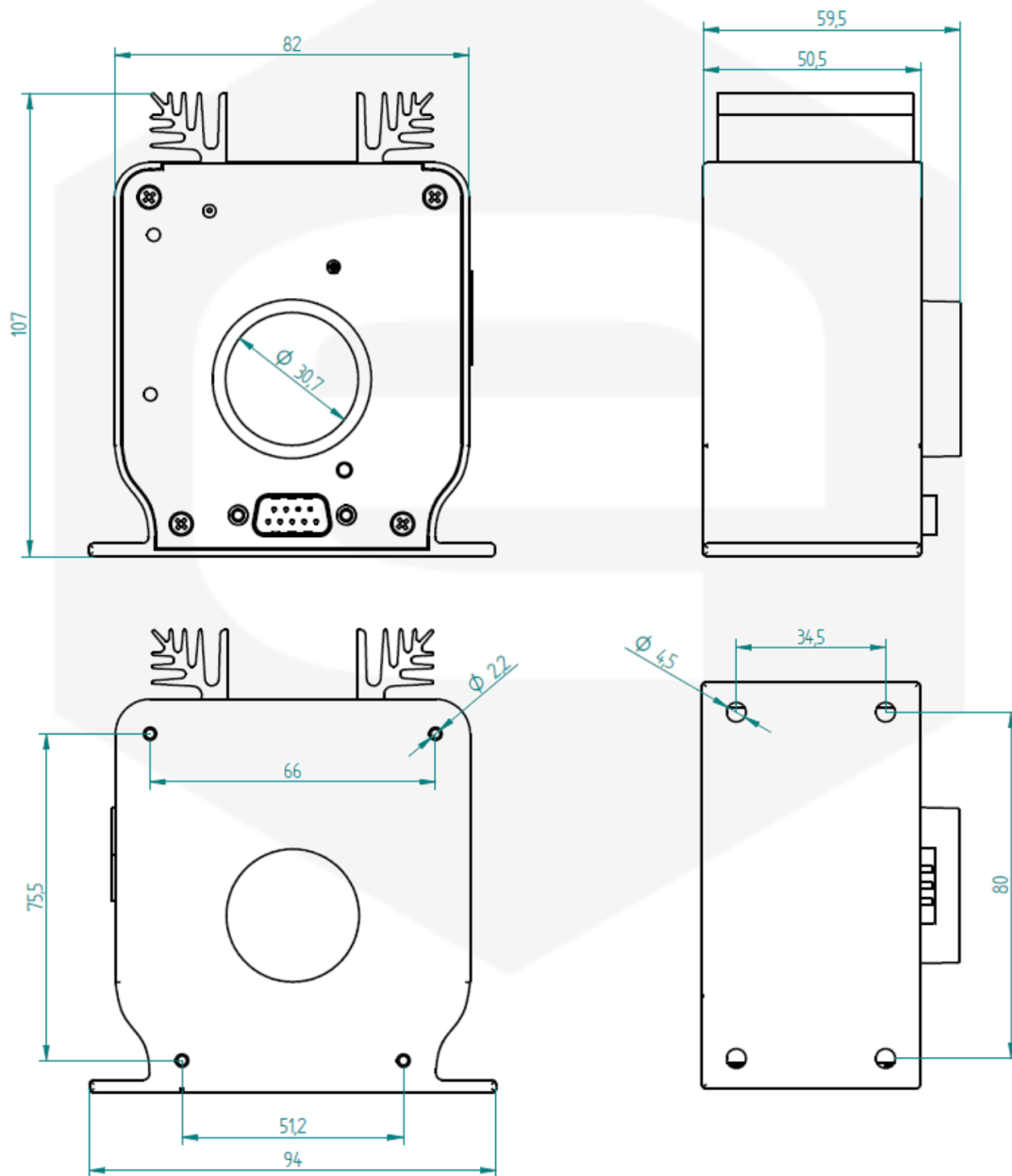
Figure 15: Mechanical drawings
