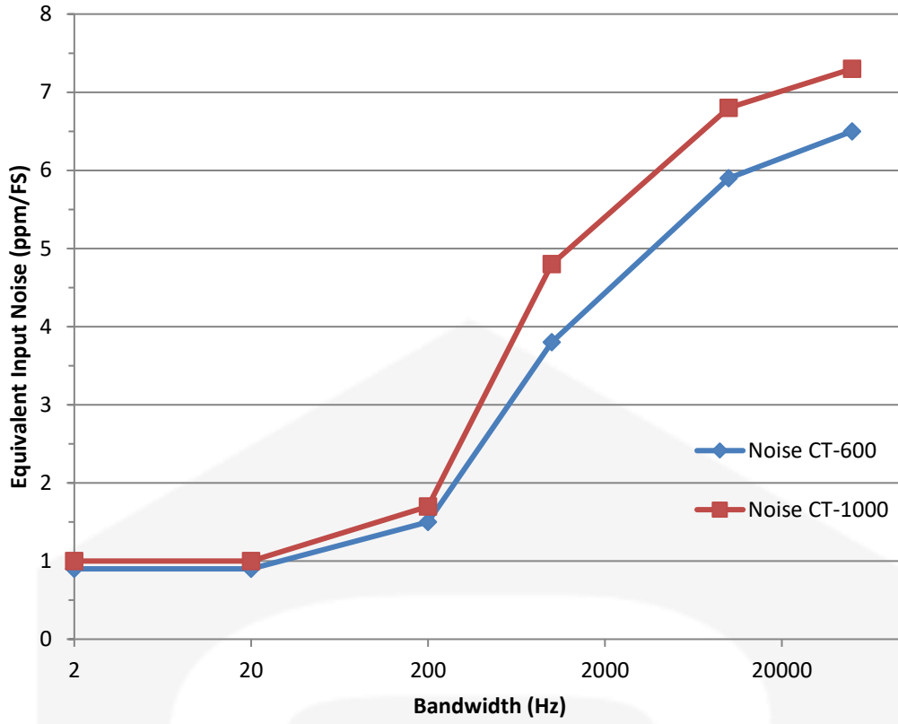
Figure 12: Equivalent input noise graph (typical values)
