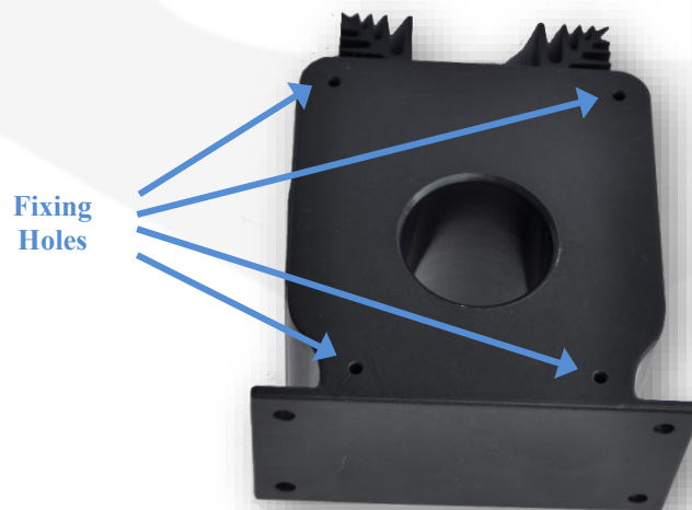
Figure 9: rear mounting holes for self-threading screws
