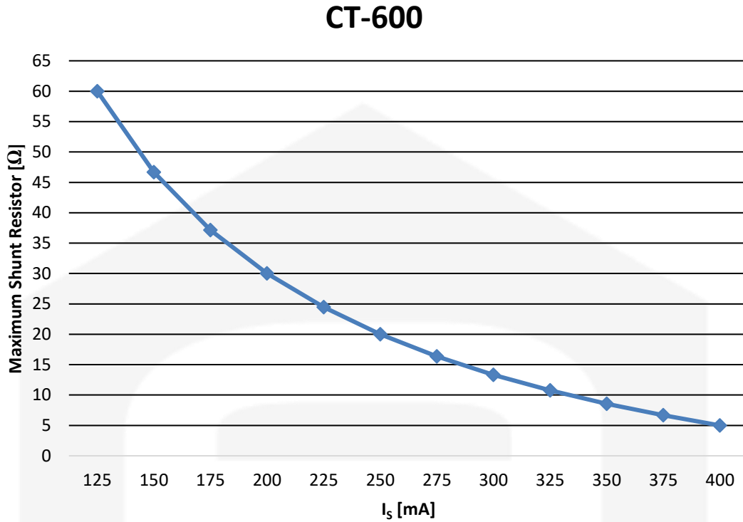
Figure 13: CT-600 maximum external shunt resistor ( Current version only)
