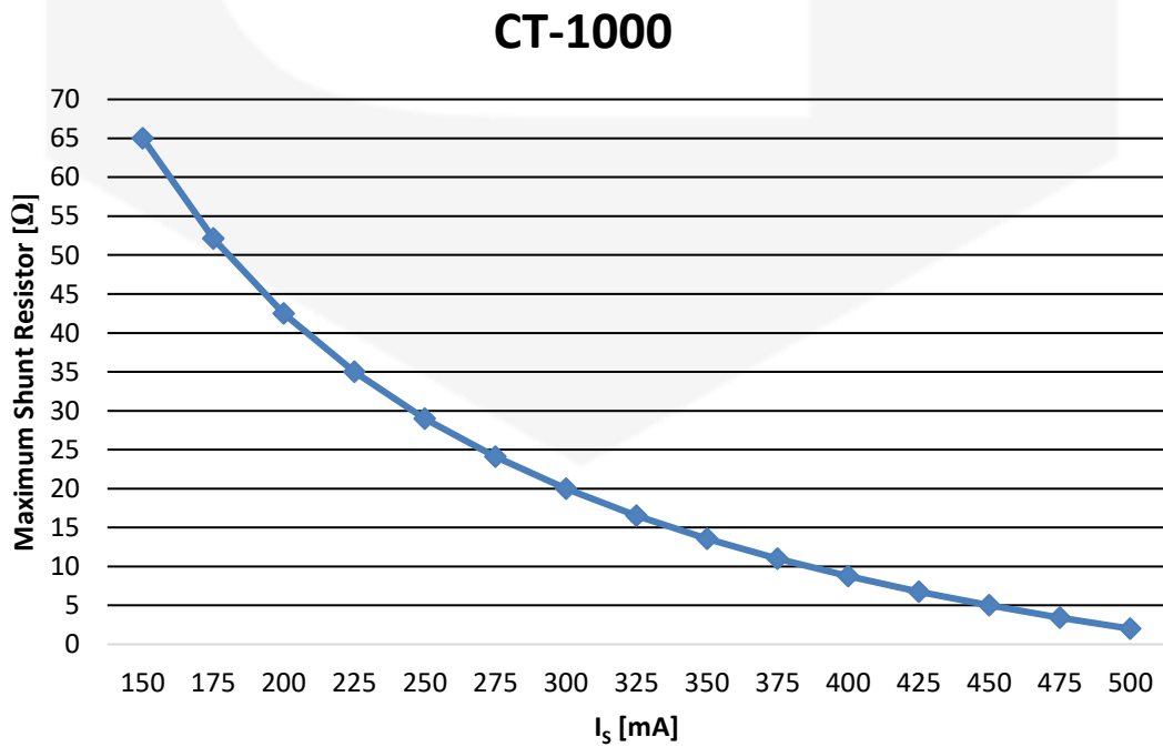
Figure 14: CT-1000 maximum external shunt resistor ( Current version only)
