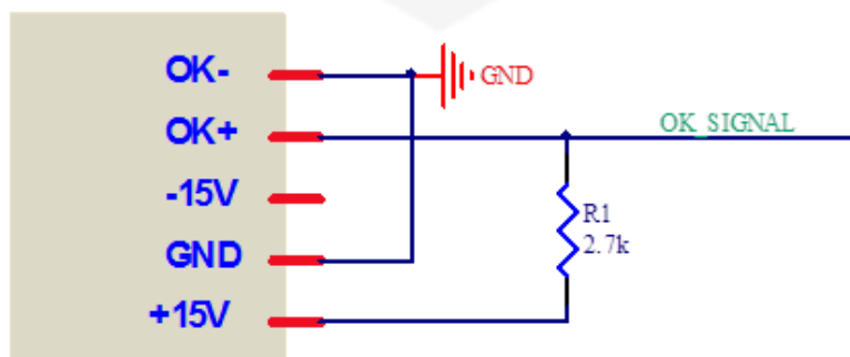
Figure 5: OUT OK signals connections using the +15V and the GND pins
