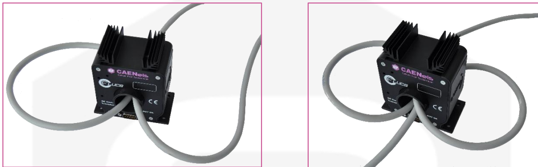
Figure 11: primary full-scale current scaled by a factor 2 (2 primary turns - left) and scaled by 3 (3 primary turns - right)
