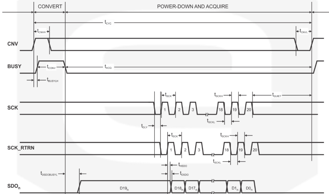
Figure 13: Timing diagram
