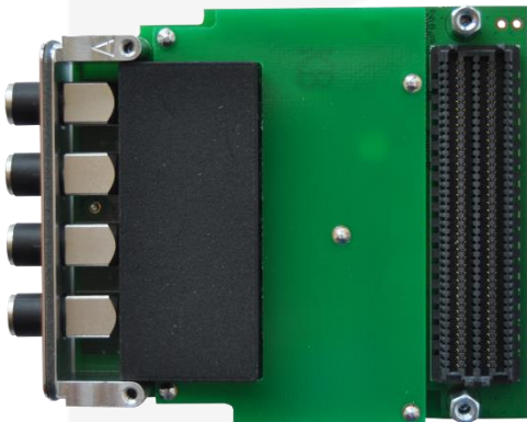
Figure 2: FMC-Pico-1M4 side 2
