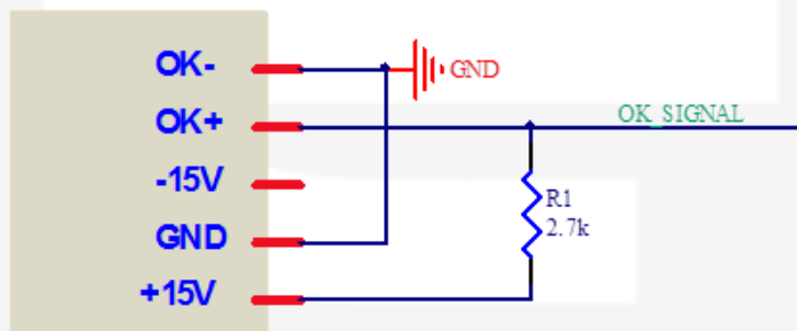
Figure 10: OUT OK signals connections using the +15V and the GND pins
