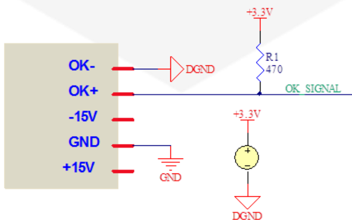
Figure 11: OUT OK signals connections as digital interfacing to +3.3V
